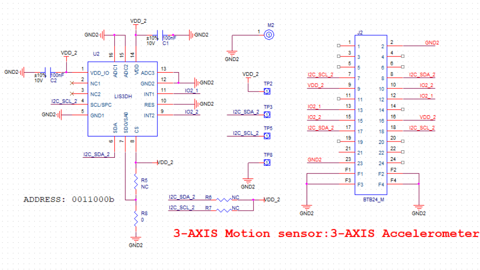
Figure 5: RAK1904 WisBlock Sensor schematics
