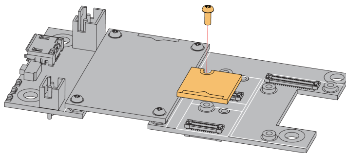
Figure 1: RAK1904 WisBlock Sensor Mounting
